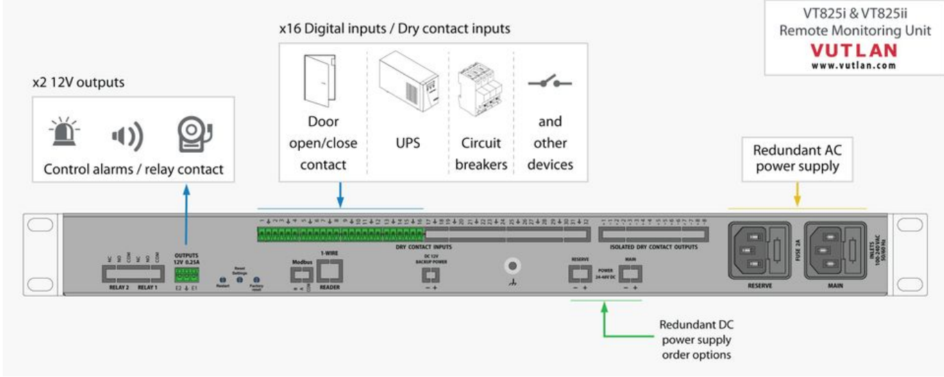
The back panel of VT825ii:
