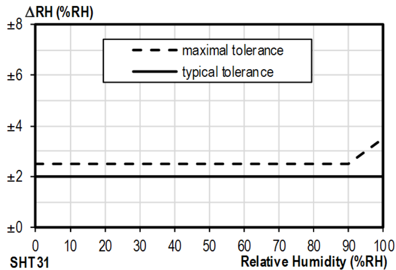
Fig. 26 – Accuracy of humidity measuring
