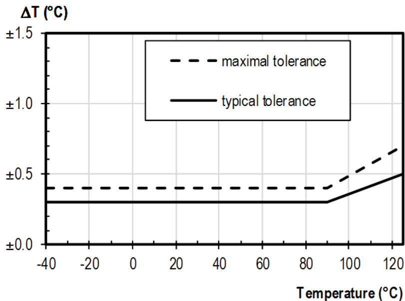
Fig. 27 – Accuracy of temperature measurement
