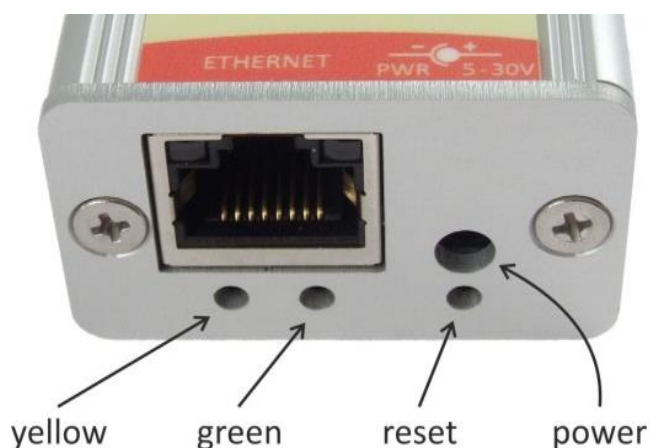
Fig. 25 – Indicators, power connector and the Ethernet connector
