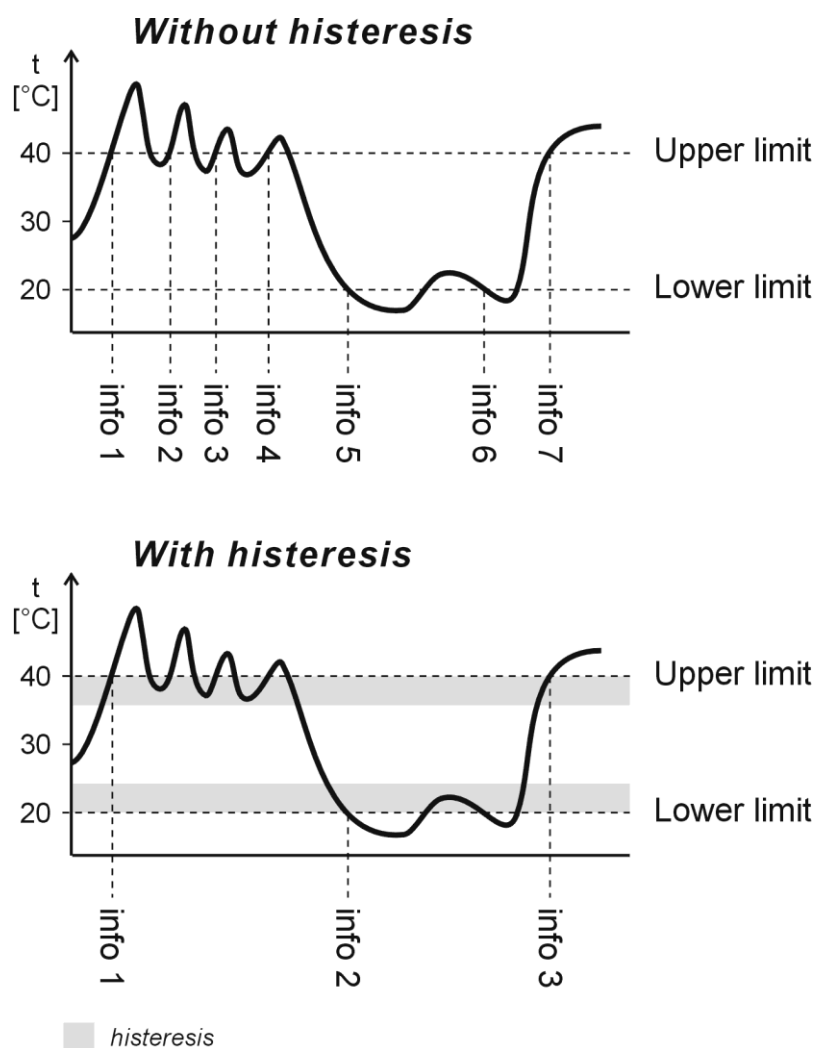
Fig. 16 – Hysteresis
