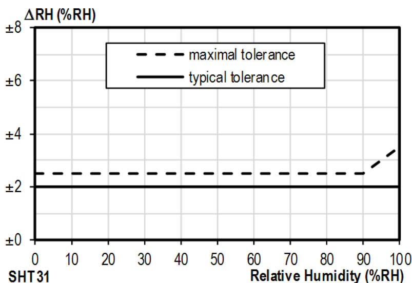
Fig. 16 – Accuracy of humidity measuring
